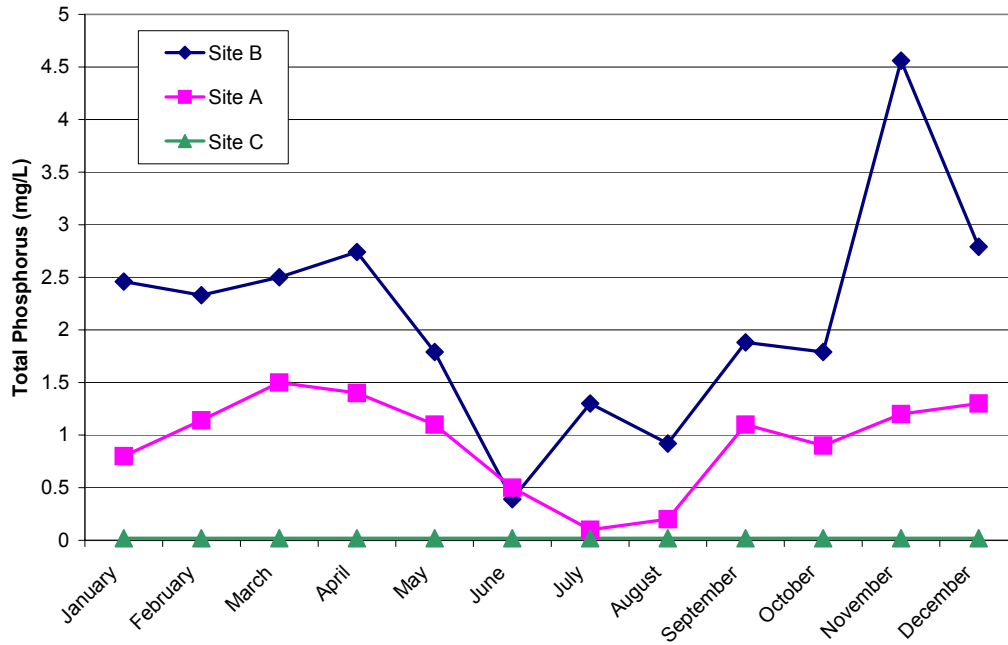
Monthly Phosphorus Measurements 2003 Trout River Watershed
