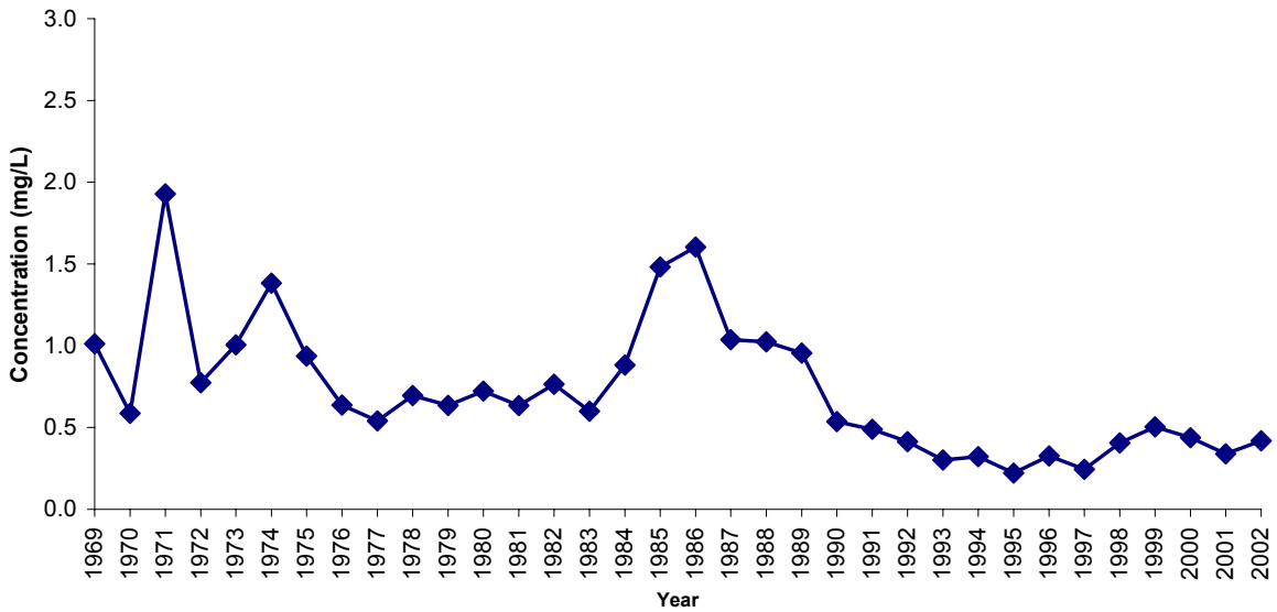
Annual Average Total Phosphorus Salmon River Watershed Site A 1969 to 2002
