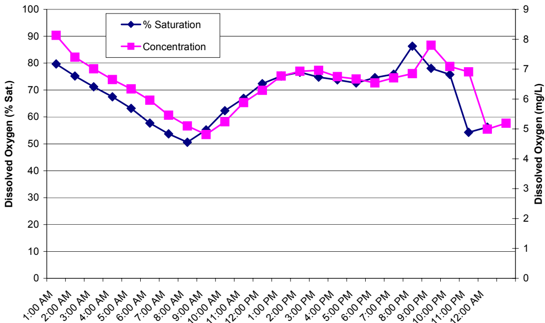
Dissolved Oxygen Measurements 2003 Trout River Watershed
